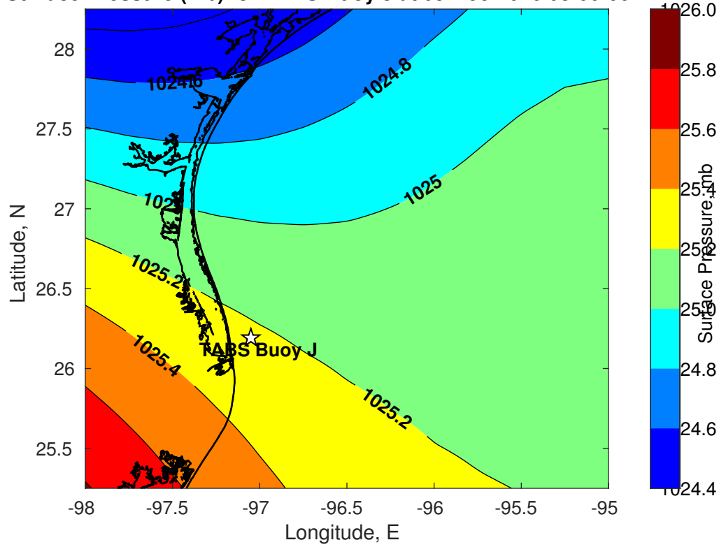
Surface Pressure (mb) for TABS Buoy J at 09-Dec-2020 03:00:00
