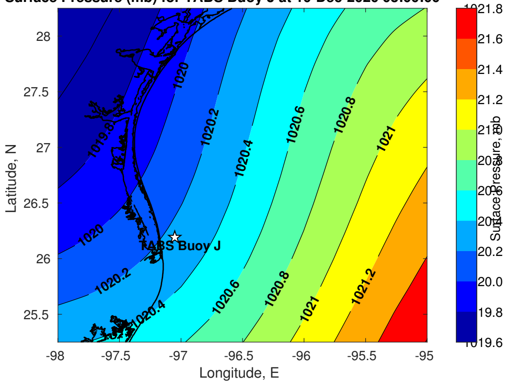
Surface Pressure (mb) for TABS Buoy J at 10-Dec-2020 03:00:00
