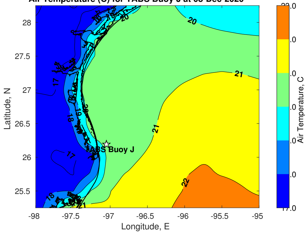
Air Temperature (C) for TABS Buoy J at 08-Dec-2020
