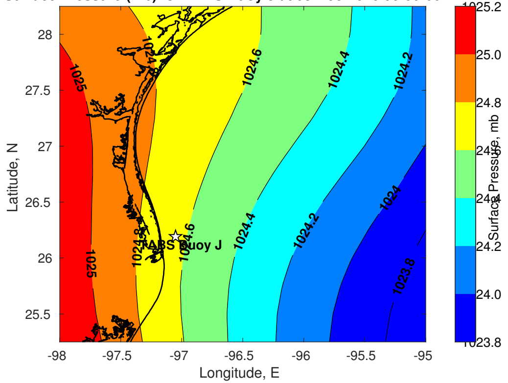
Surface Pressure (mb) for TABS Buoy J at 08-Dec-2020 06:00:00
