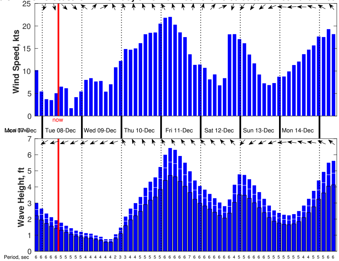
Wind & Wave Forecast for TABS Buoy J from 07-Dec-2020 19:00:00 to 15-Dec-2020 07:00:00
