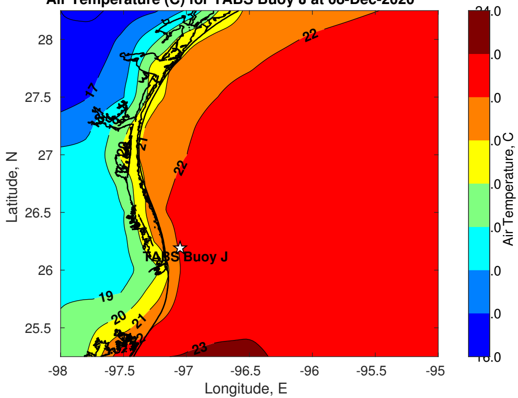
Air Temperature (C) for TABS Buoy J at 08-Dec-2020
